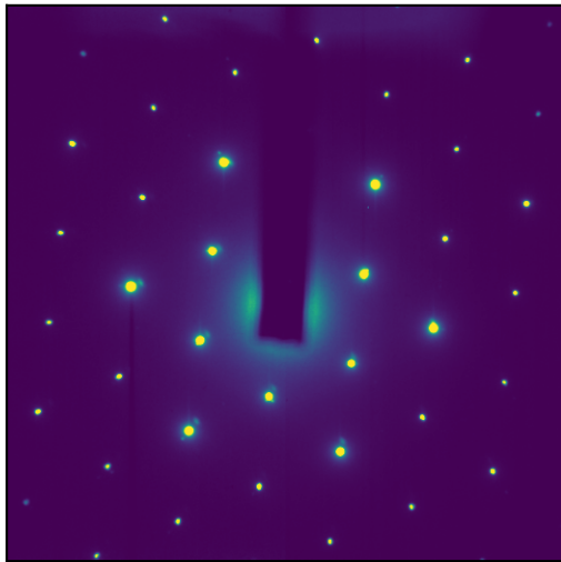
Graphite
