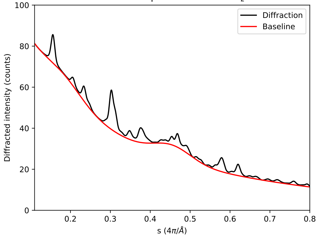
Diffraction pattern of rutile \text{VO}_2
