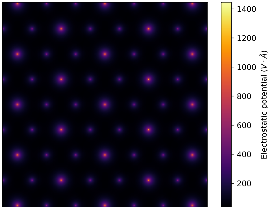
Electrostatic potential of graphite
