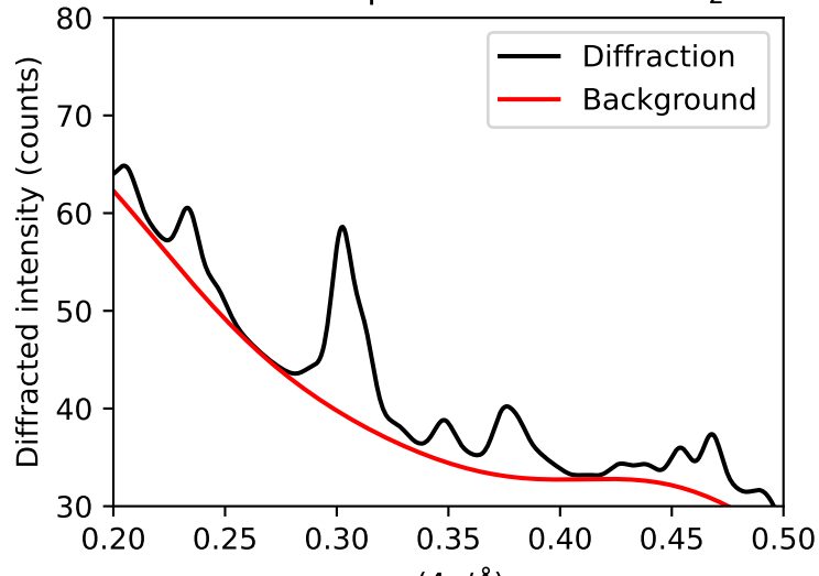
Diffraction pattern of rutile VO 2
