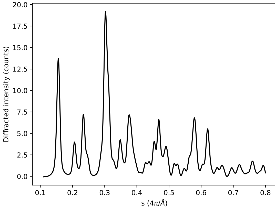
Background-subtracted diffraction pattern of rutile VO 2
